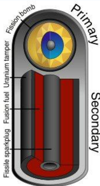
(Picture Below - Teller-Ulam Fusion Device)
